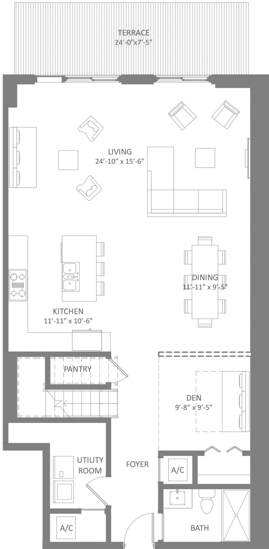
GROUND FLOOR
